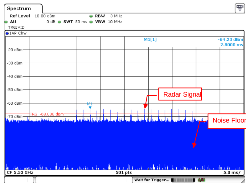
Radar Signal 0
