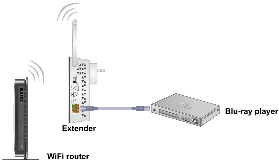
Figure 4. Ethernet connection to the extender
