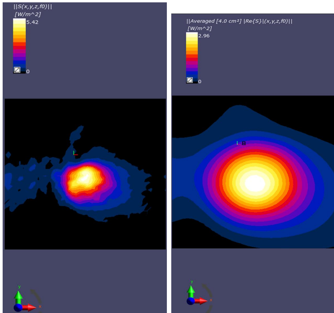
Figure 4-1 Band 260, beam ID 6, pointPD and 4cm²PD , Front
