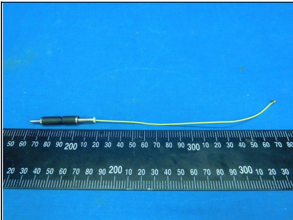
Antenna: 2.4GHz_Chain 3
