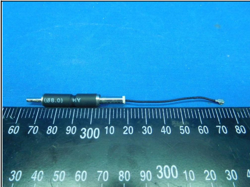
Antenna: 2.4GHz_Chain 1
