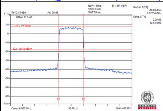
802.11ax (HE80)_Chain 3 / CH183 (U-NII-8 Band)
