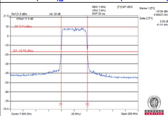
802.11ax (HE40)_Chain 2 / CH211 (U-NII-8 Band)
