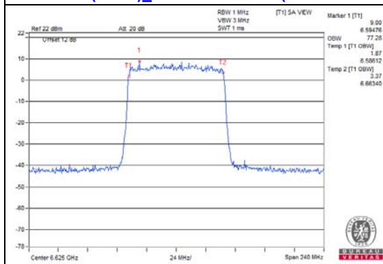
802.11ax (HE80)_Chain 3 / CH135 (U-NII-7 Band)
