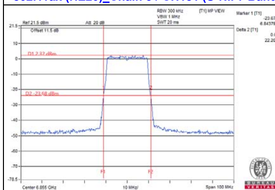
802.11ax (HE20)_Chain 3 / CH181 (U-NII-7 Band)
