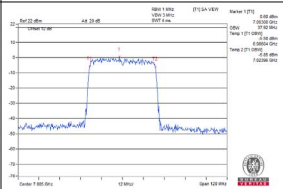
802.11ax (HE40)_Chain 2 / CH211 (U-NII-8 Band)
