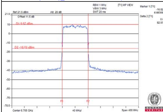
802.11ax (HE80)_Chain 2 / CH151 (U-NII-7 Band)
