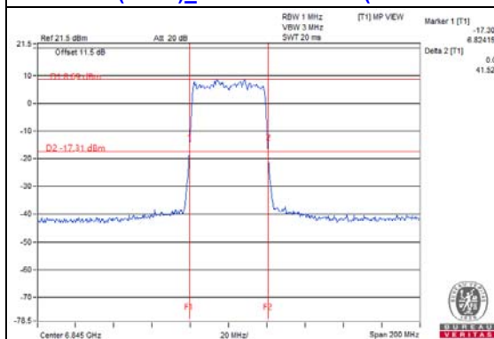
802.11ax (HE40)_Chain 3 / CH179 (U-NII-7 Band)
