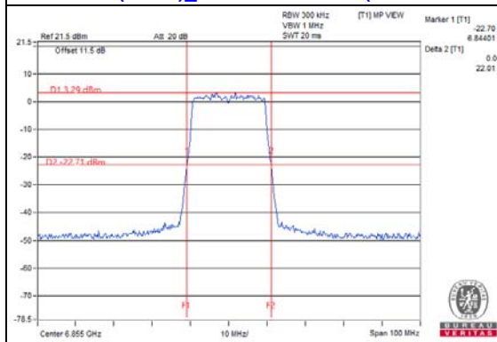
802.11ax (HE20)_Chain 2 / CH181 (U-NII-7 Band)
