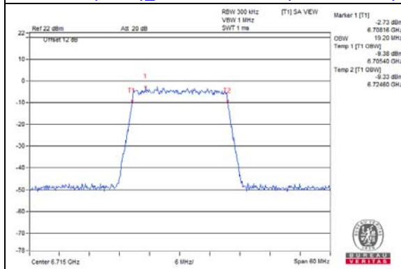
802.11ax (HE20)_Chain 0 / CH153 (U-NII-7 Band)
