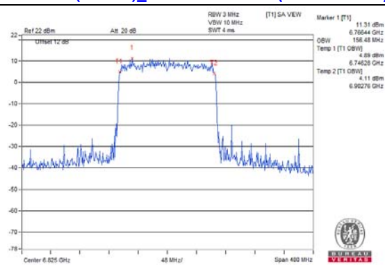
802.11ax (HE160)_Chain 0 / CH175 (U-NII-8 Band)
