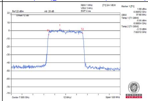
802.11ax (HE40)_Chain 1 / CH211 (U-NII-8 Band)
