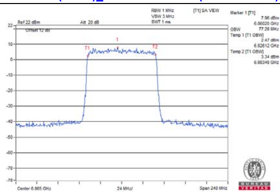
802.11ax (HE80)_Chain 0 / CH183 (U-NII-8 Band)
