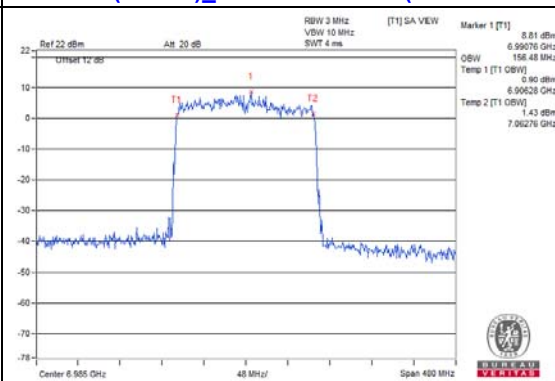
802.11ax (HE160)_Chain 1 / CH207 (U-NII-8 Band)
