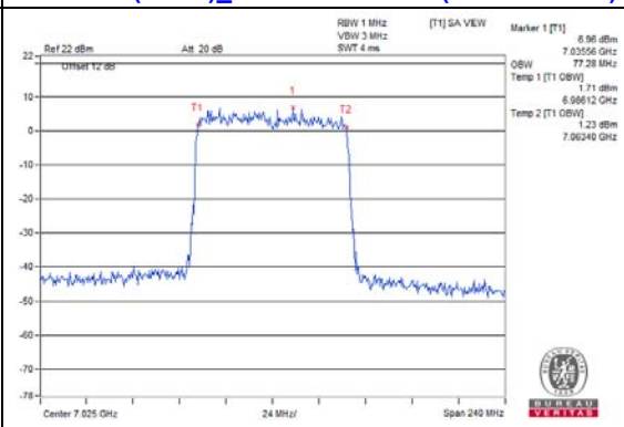
802.11ax (HE80)_Chain 3 / CH215 (U-NII-8 Band)
