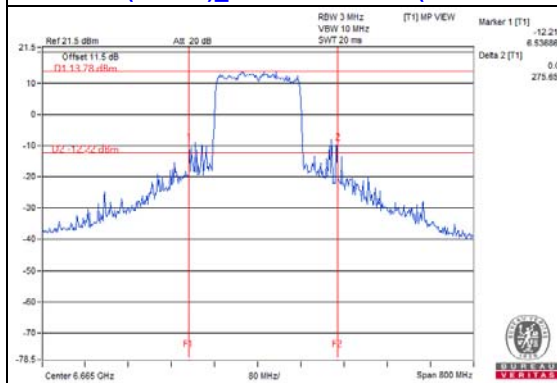
802.11ax (HE160)_Chain 3 / CH143 (U-NII-7 Band)
