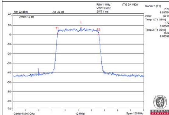
802.11ax (HE40)_Chain 2 / CH179 (U-NII-7 Band)
