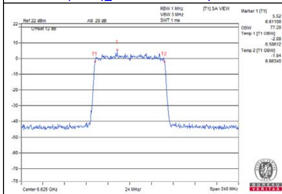
802.11ax (HE80)_Chain 0 / CH135 (U-NII-7 Band)
