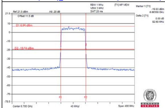
802.11ax (HE80)_Chain 2 / CH151 (U-NII-7 Band)
