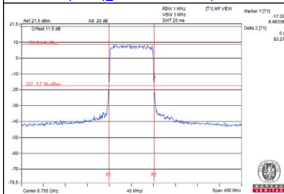
802.11ax (HE80)_Chain 0 / CH151 (U-NII-7 Band)
