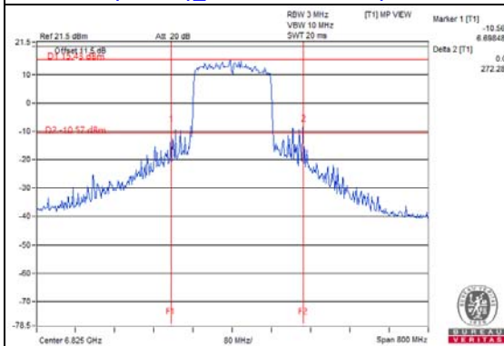
802.11ax (HE160)_Chain 1 / CH175 (U-NII-7 Band)
