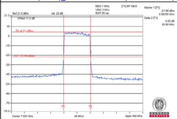
802.11ax (HE80)_Chain 3 / CH215 (U-NII-8 Band)
