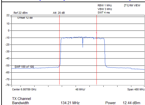
802.11ax (HE160)_Chain 0 / CH175 (U-NII-7 Band)
