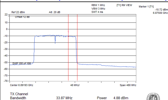
802.11ax (HE160)_Chain 0 / CH175 (U-NII-8 Band)
