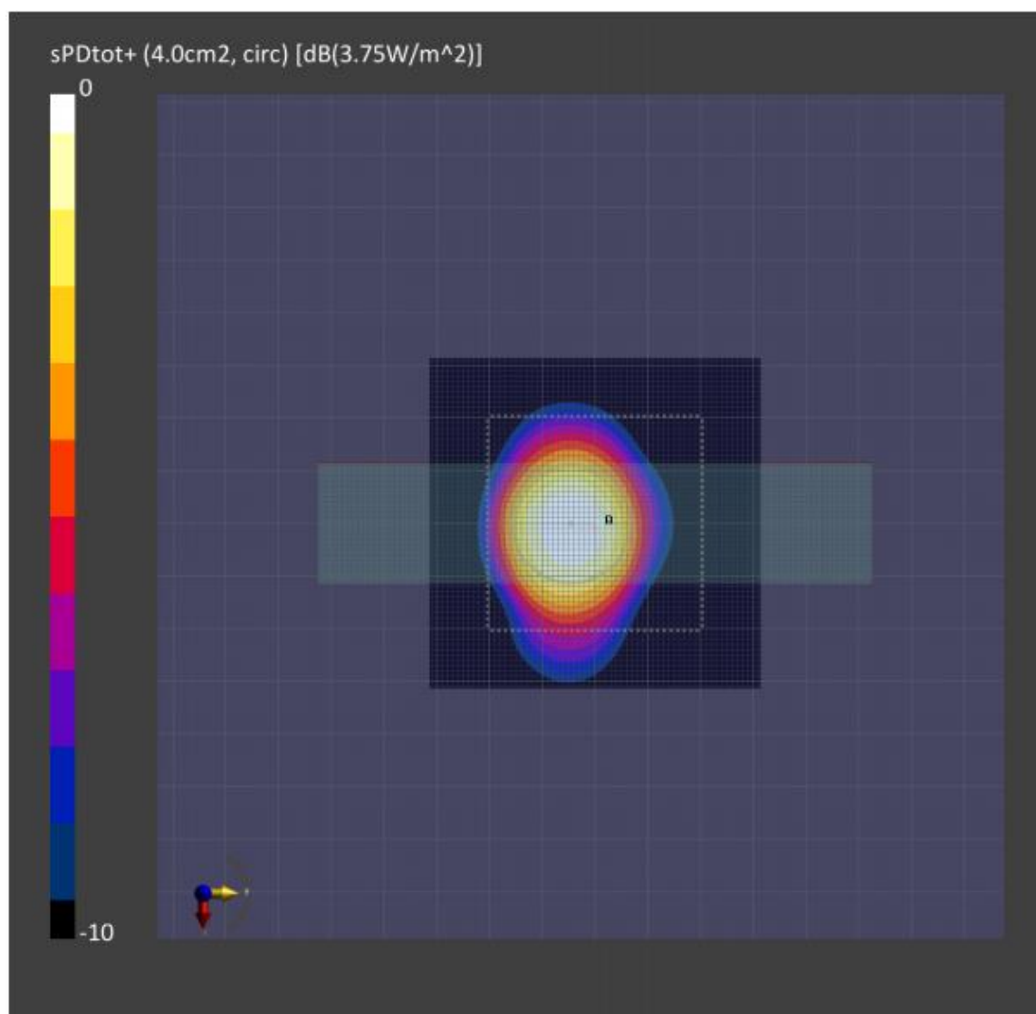
Figure8-3: 4cm 2 -averaged power density distribution measured at input.power.limit of 3.75dBm on the Right Side for n260 beam 36
