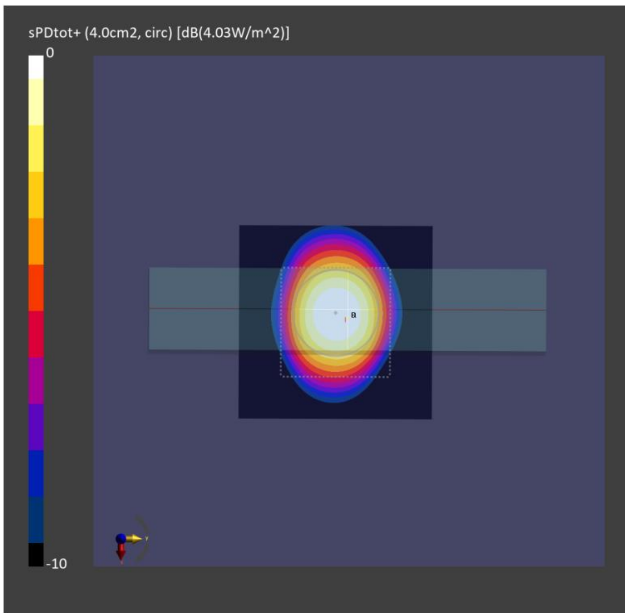
Figure8-2: 4cm 2 -averaged power density distribution measured at input.power.limit of 4.03dBm on the Right Side for n260 beam 36
