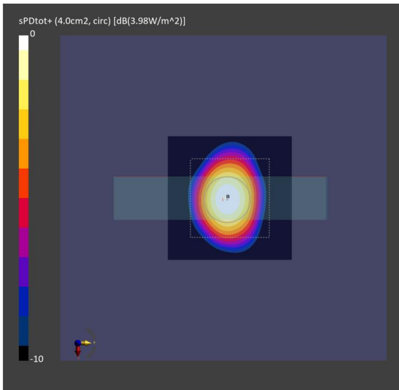
Figure8-3: 4cm 2 -averaged power density distribution measured at input.power.limit of 3.98dBm on the Left Side for n261 beam 39
