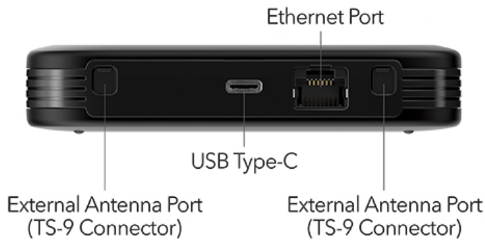
Figure 2. Nighthawk M6 connectors
