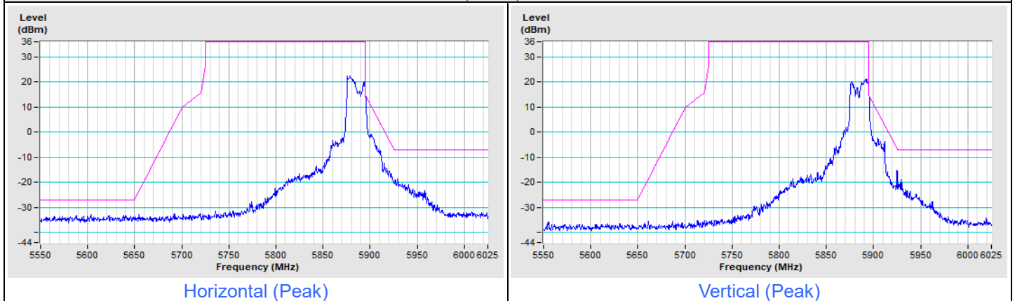
802.11ax (HE20) Channel 177
