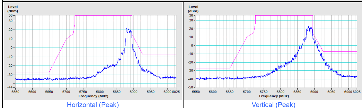
802.11a Channel 177
