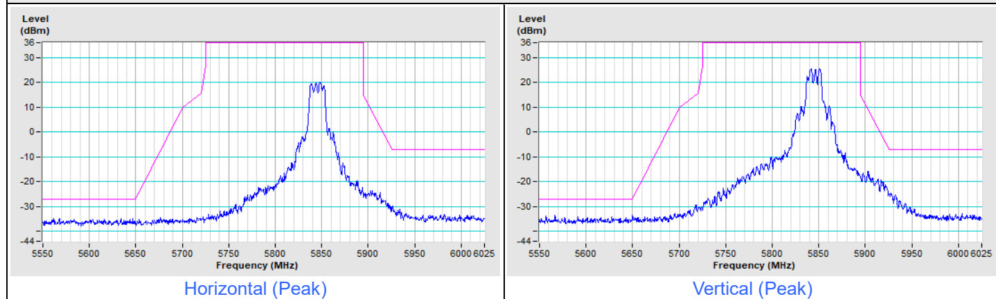
802.11a Channel 169
