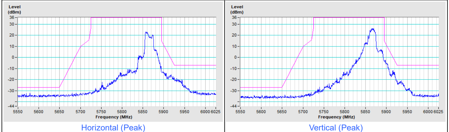
802.11ax (HE20) Channel 173
