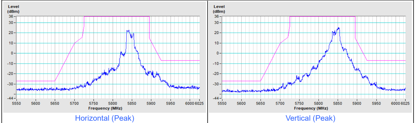
802.11ax (HE20) Channel 169
