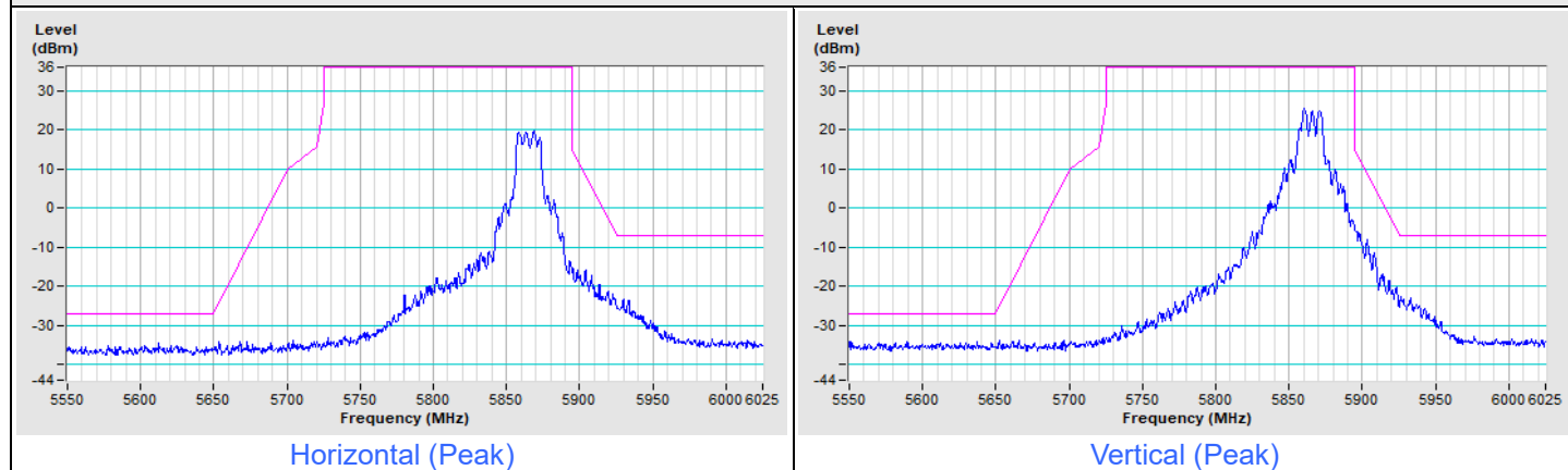
802.11a Channel 173
