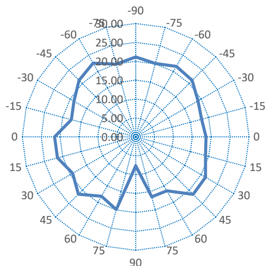
5G Ch157
