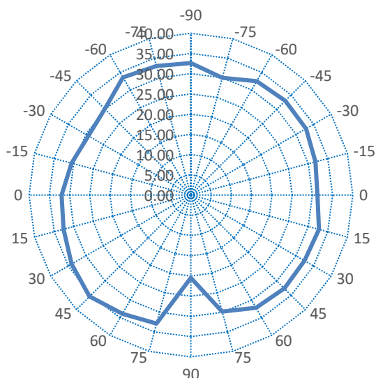
5G Ch157
