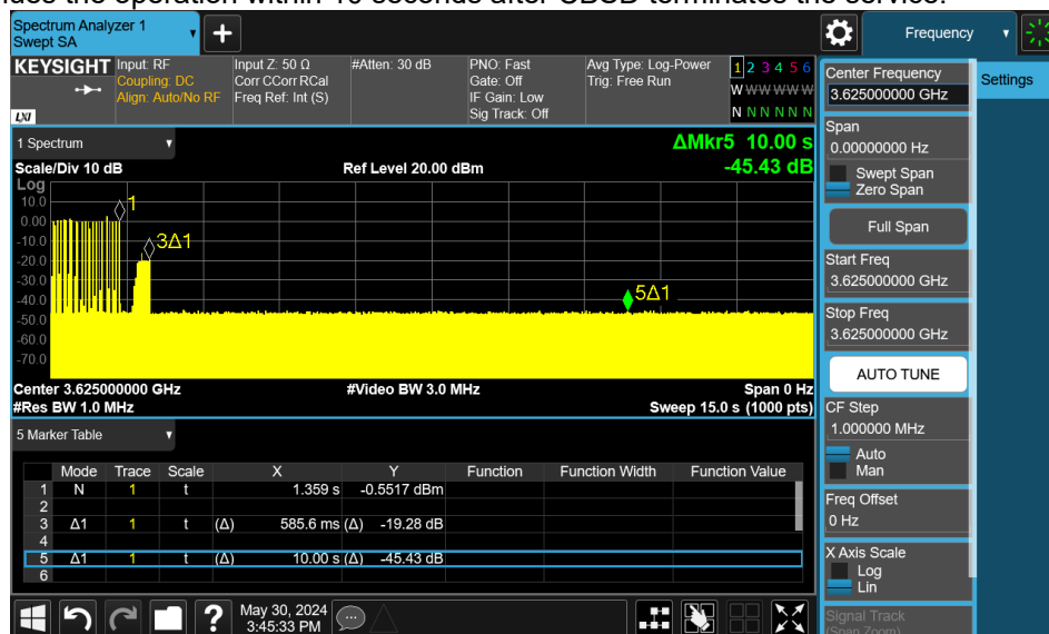
Plot 5-2 EUD discontinues operations within 10s
