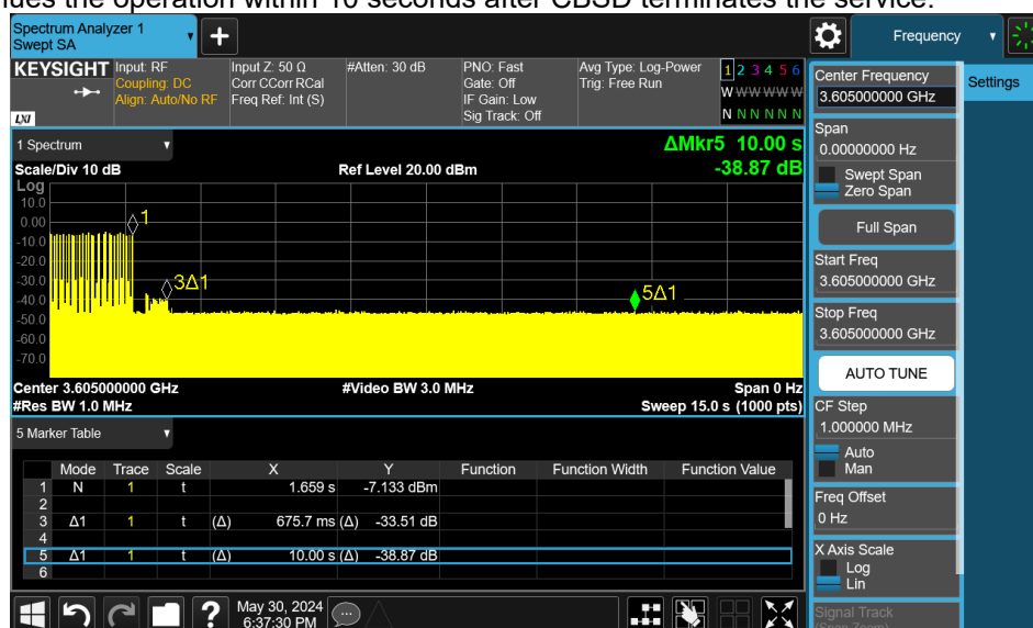
Plot 5-5 EUD discontinues operations within 10s.
