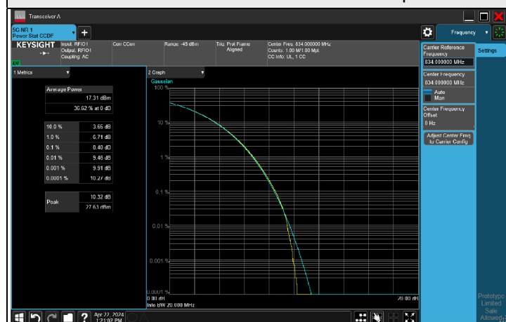
256QAM CH 166800 (834 MHz)
