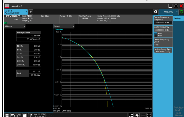
256QAM CH 167300 (836.5 MHz)
