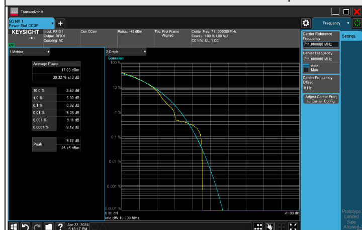
256QAM CH 142200 (711 MHz)
