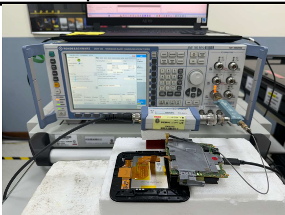
Setup for Conducted Power Test (for LTE Band)
