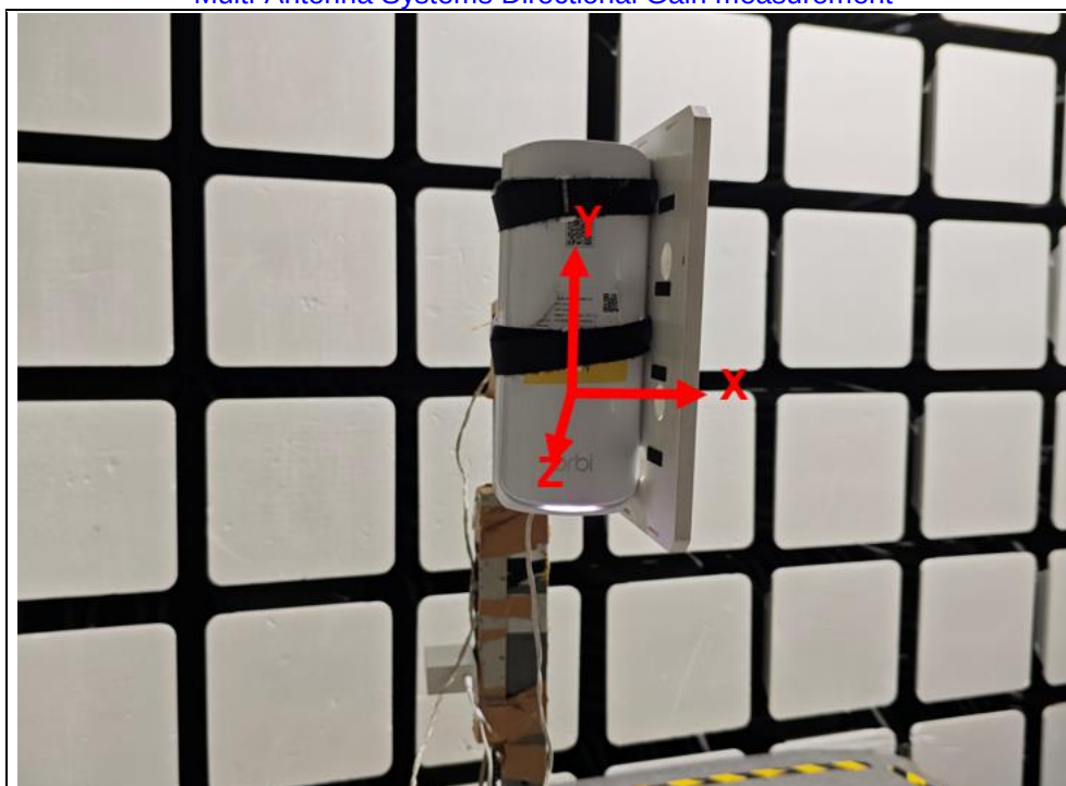
Multi-Antenna Systems Directional Gain measurement
