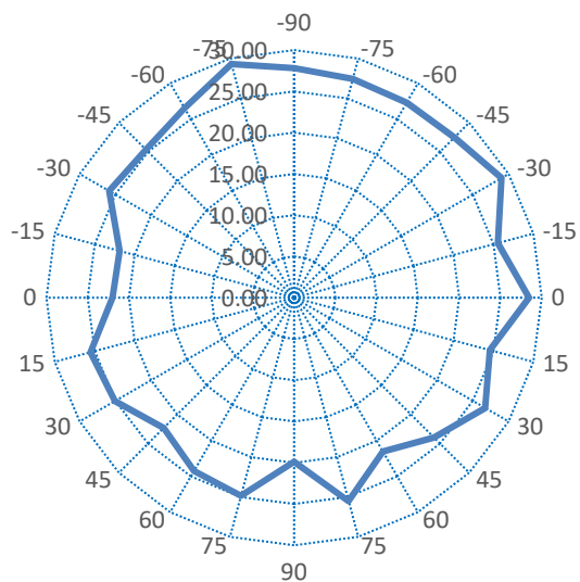
5G Ch157
