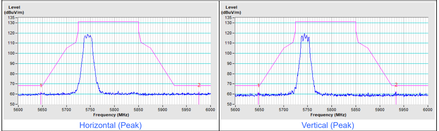
802.11a Channel 149
