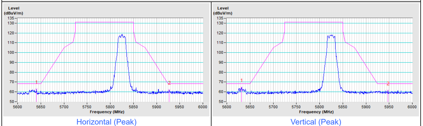
802.11a Channel 165
