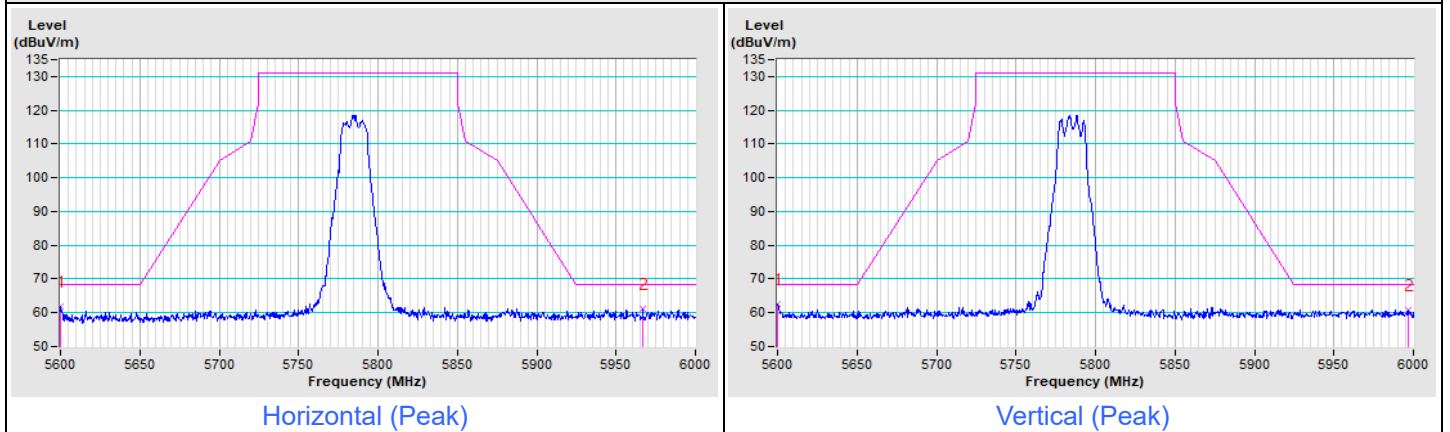
802.11a Channel 157
