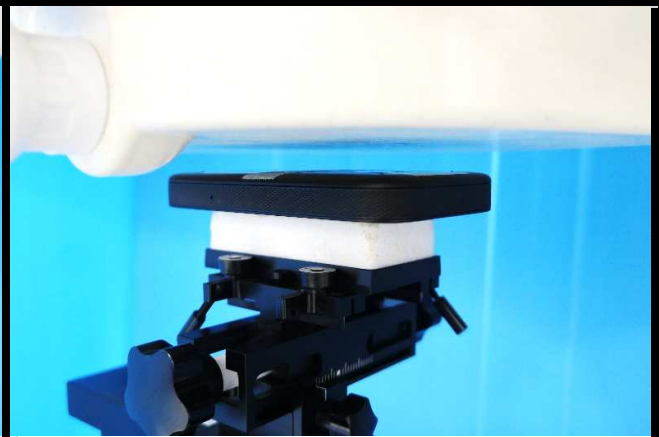
Rear Face of EUT Tested at 13 mm
