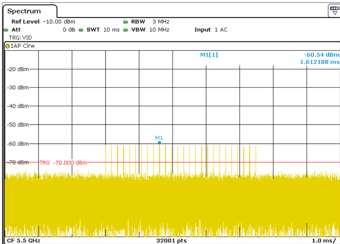
Radar Signal 2
