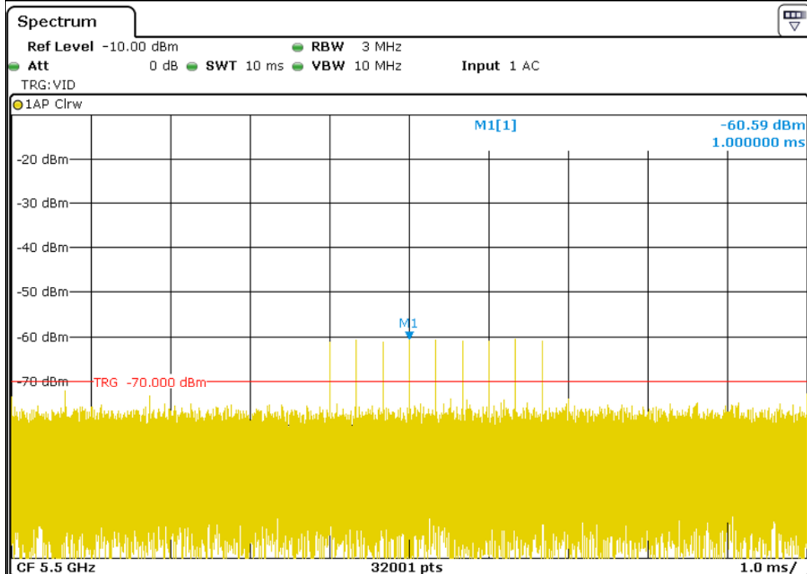
Radar Signal 6
