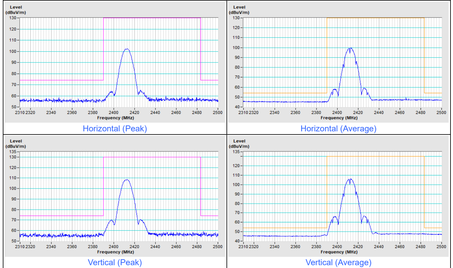
802.11b Channel 1
