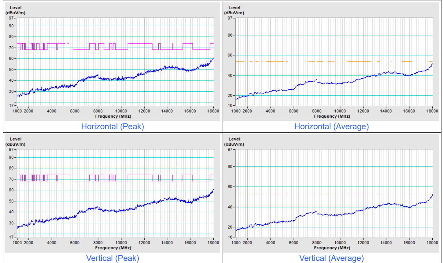
802.11a Channel 140
