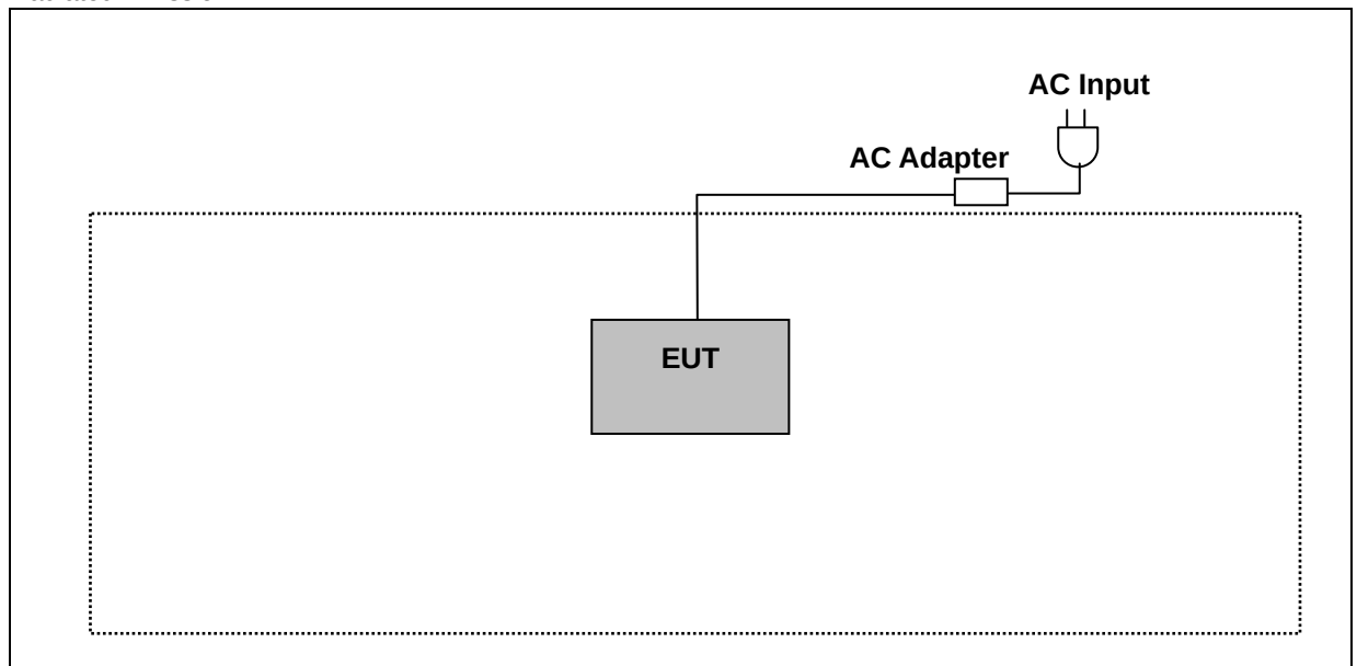
Radiated Emission
