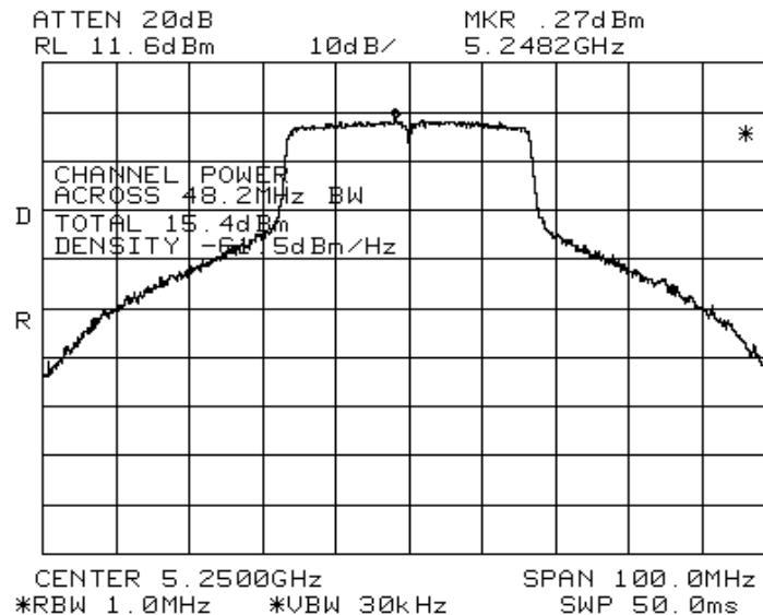
Spectrum Analyzer channel power @ 5.25 GHz
