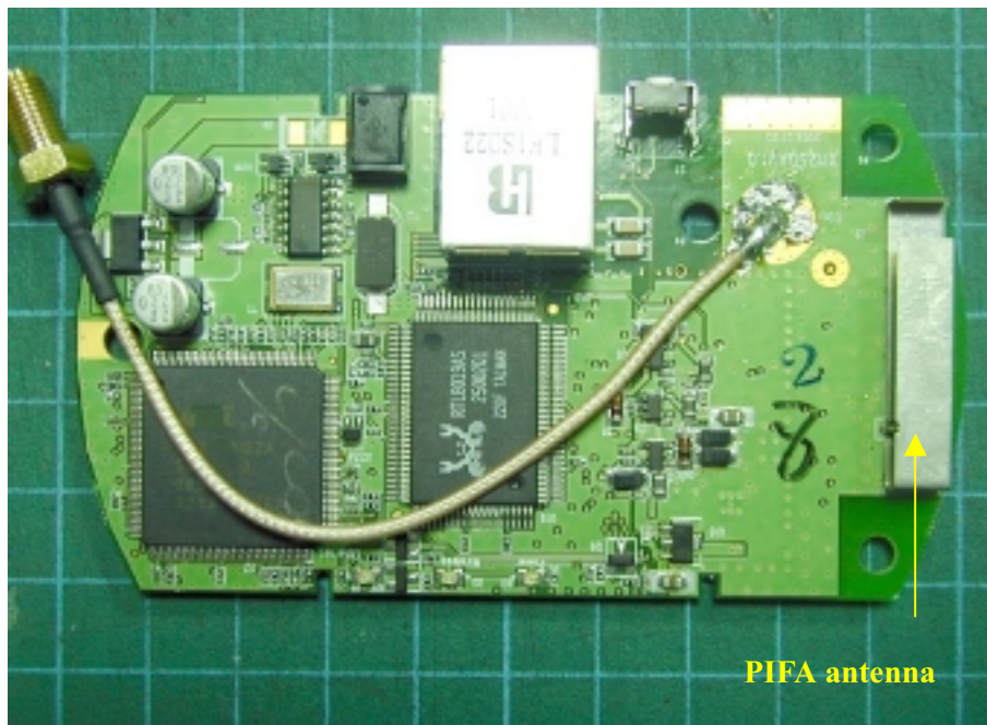
Photo 4: Photo of antenna (2dBi)
