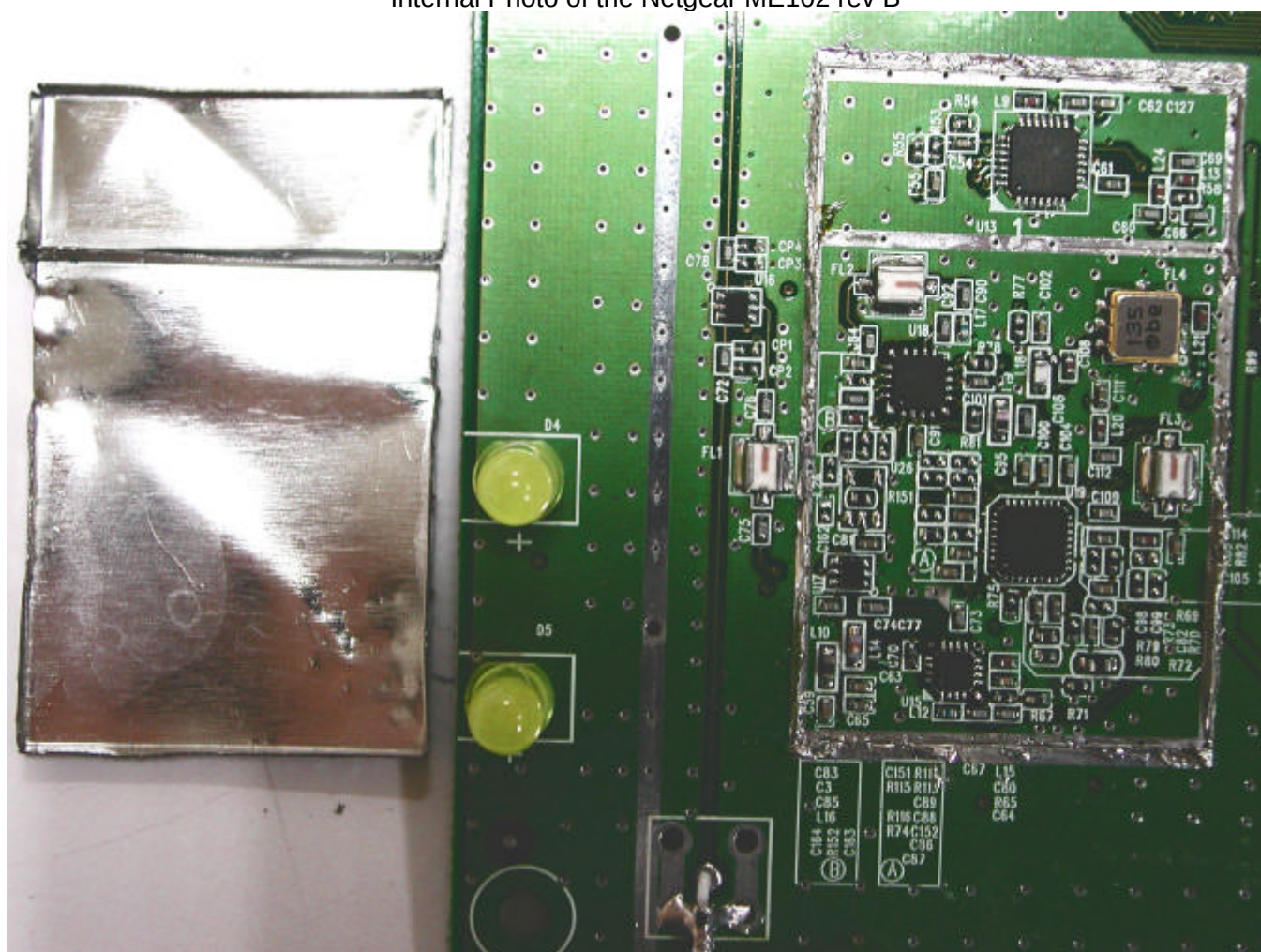
Internal Photo of the Netgear ME102 rev B
