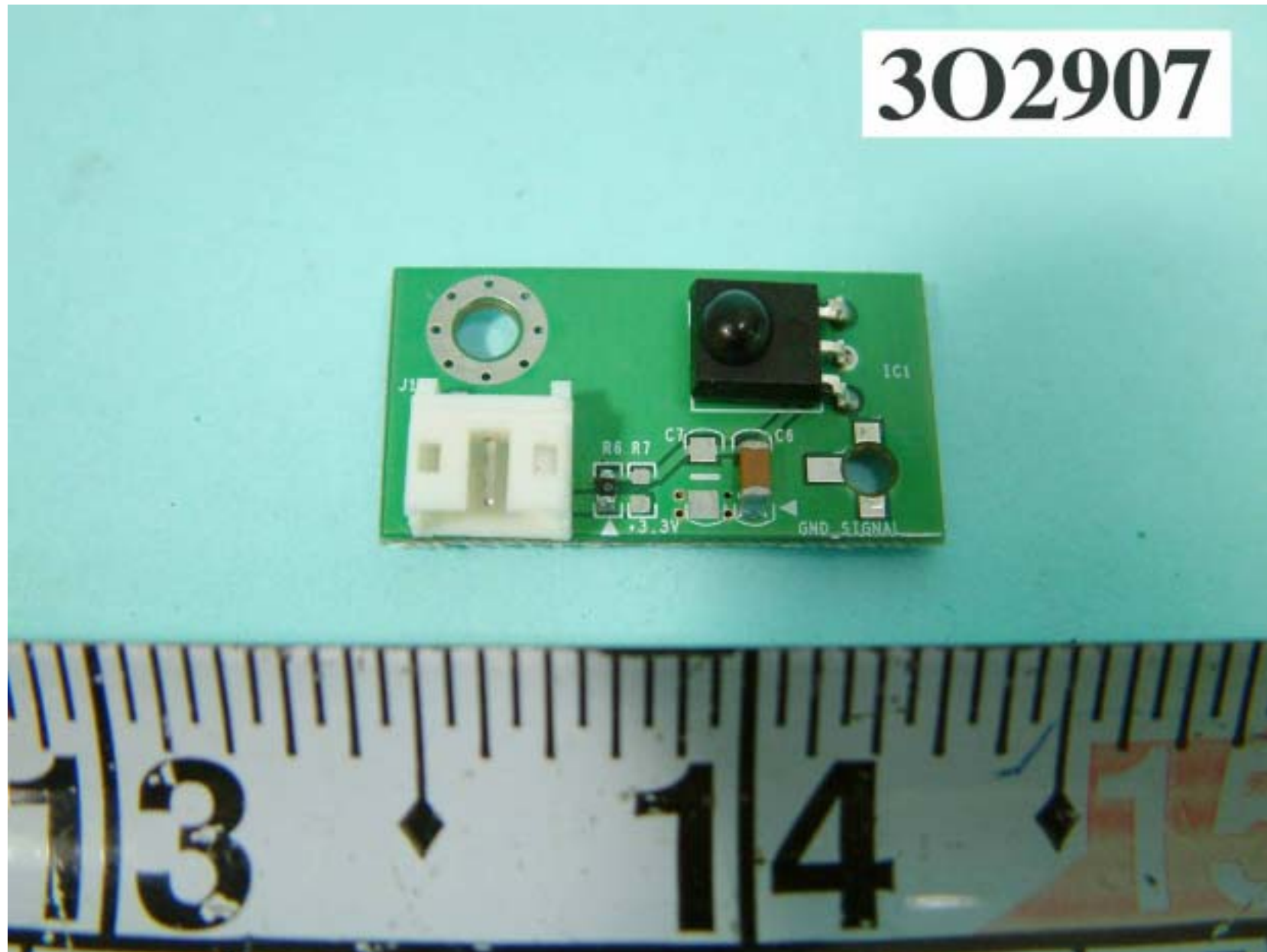
FRONT SIDE OF DAUGHTER BOARD
