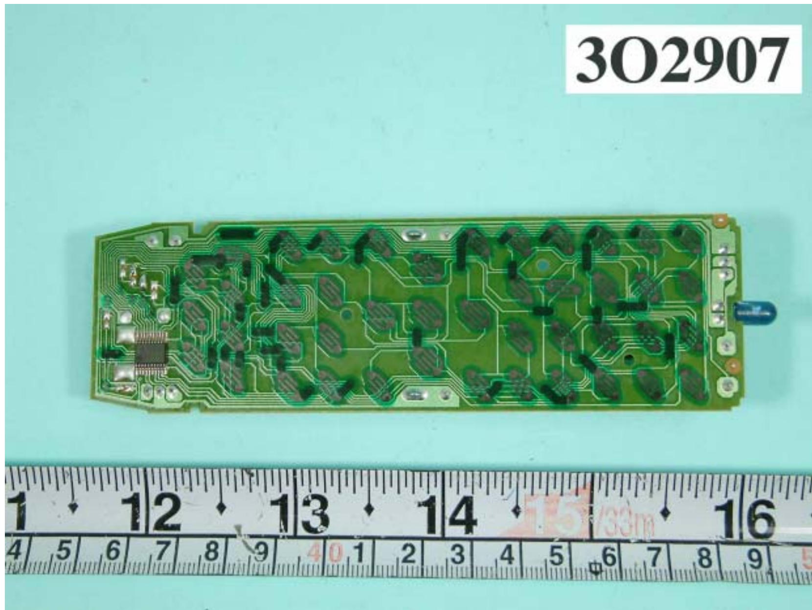
FRONT SIDE OF MAIN BOARD OF REMOTER CONTROL
