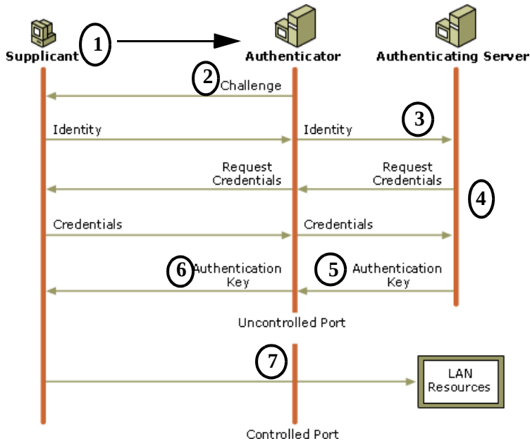
Figure D-2: 802.1x Authentication Sequence
