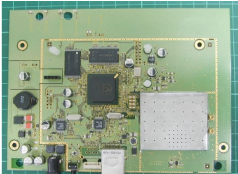
Photo 10: Inner view
