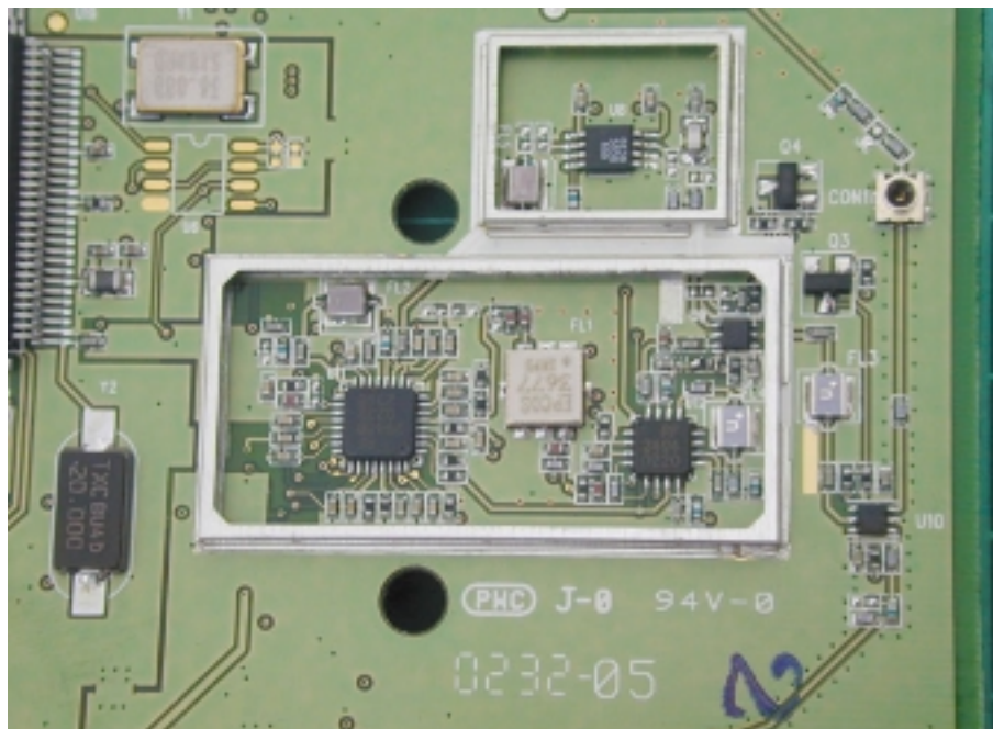
Photo 7: Inner view
