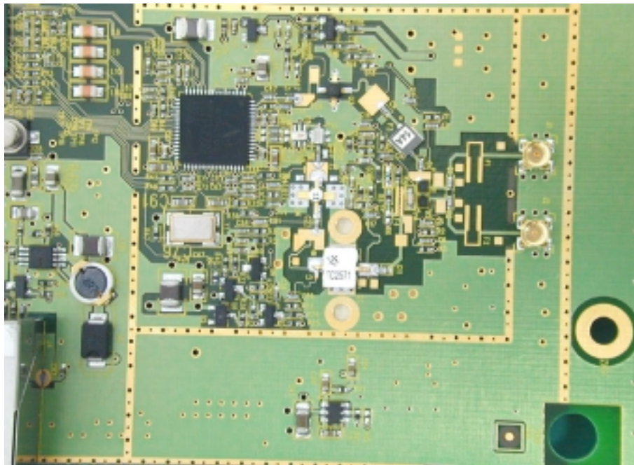
Photo 12: Inner view
