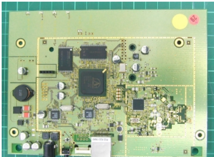
Photo 11: Inner view
