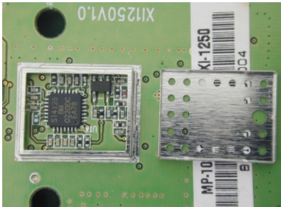
Photo 9: Inner view
