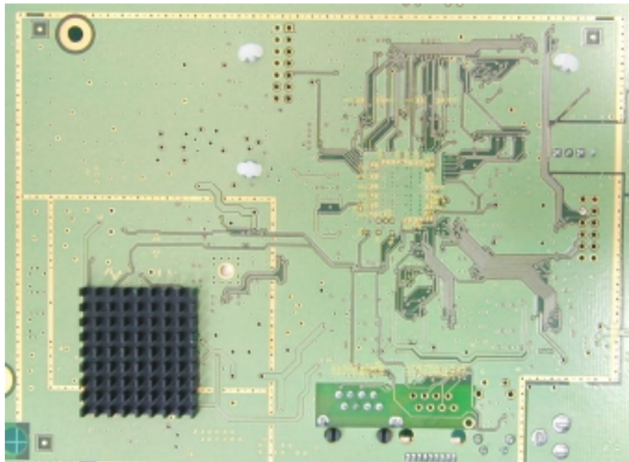
Photo 13: Inner view
