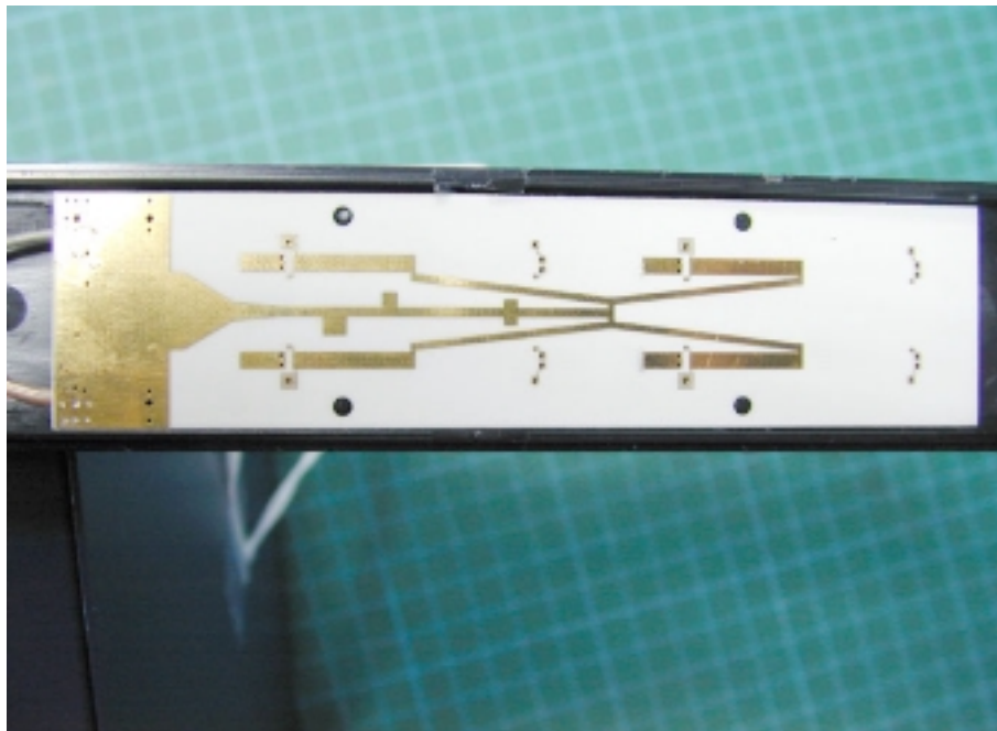
Photo 2: Antenna photo
