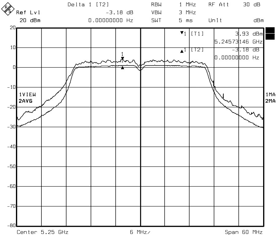
Channel Middle
