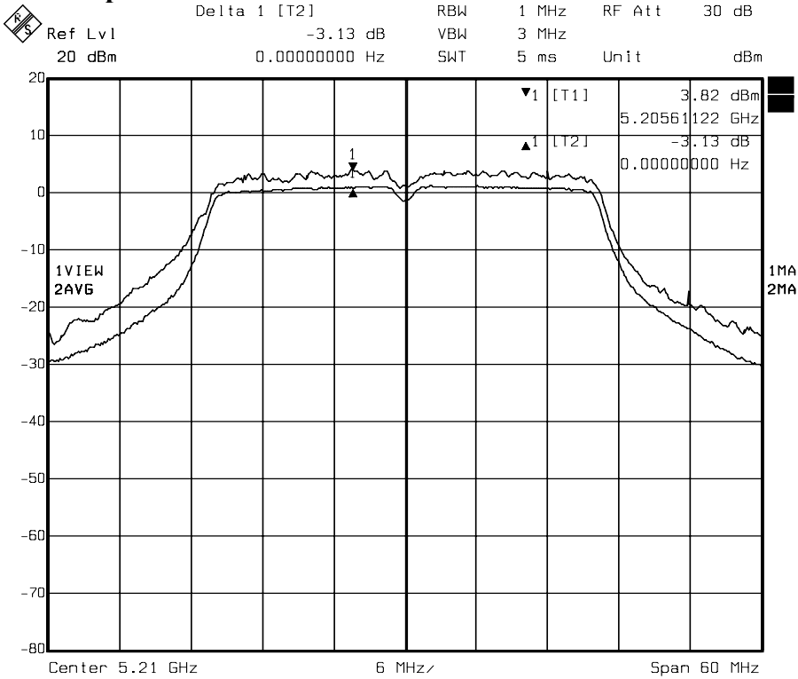
Channel Low
