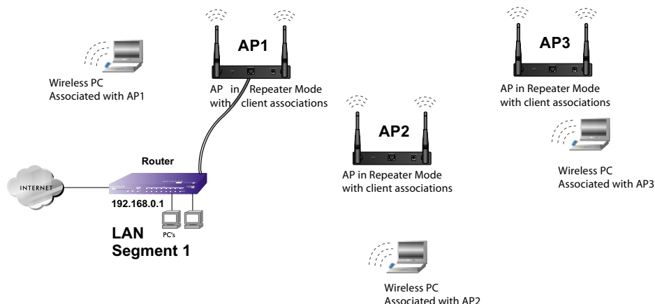
Figure 5-9: Multi-Point bridging
