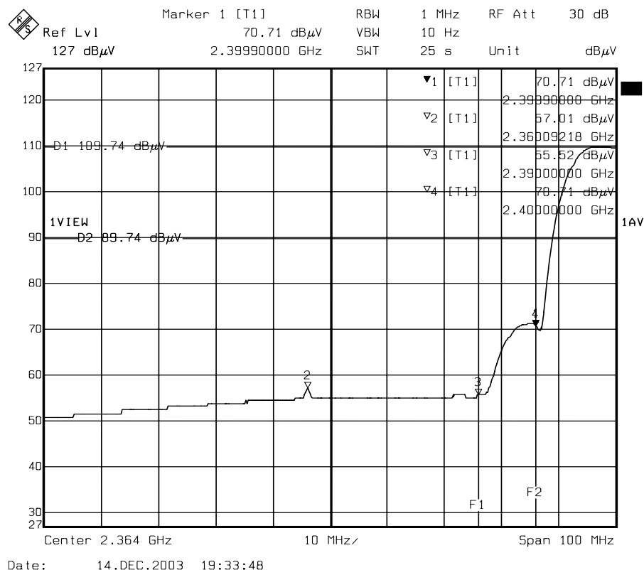
Channel 1 AVG Note: For 802.11b Mode
