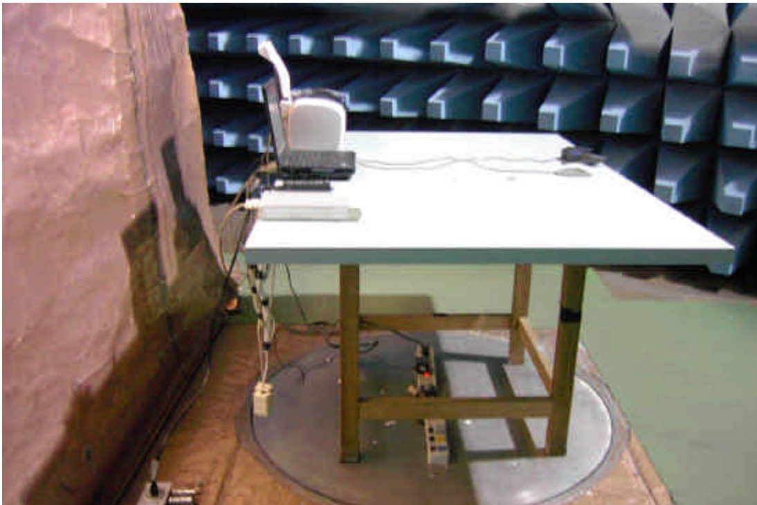
Side View of the Test Configuration
