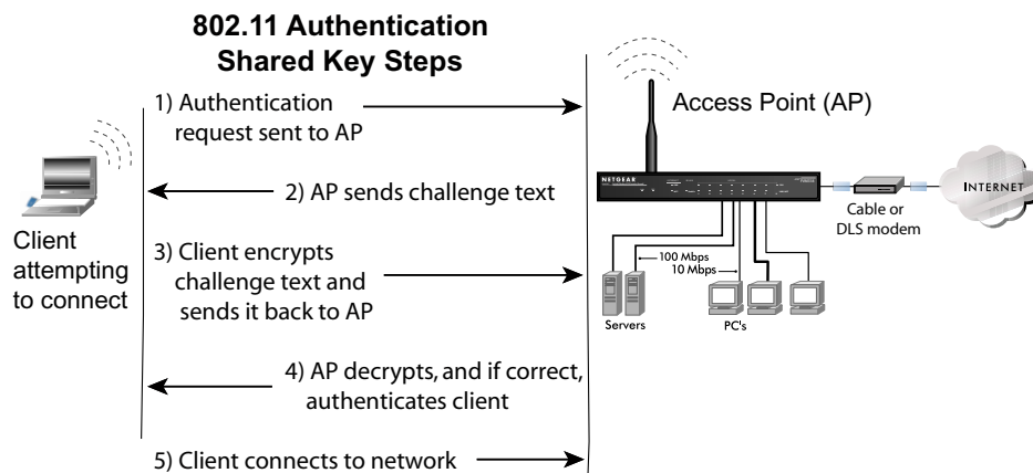
Figure 3-10: 802.11 shared key authentication
