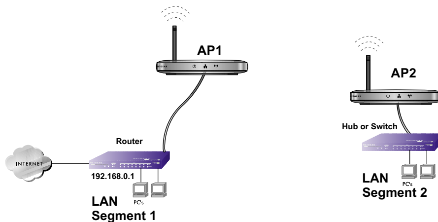
Figure 5-3: Wireless Bridging
