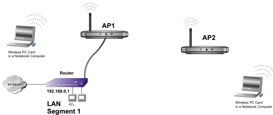
Figure 5-2: Wireless Repeater
