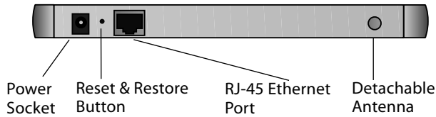
Figure 2-2: WG602 v3 rear panel
