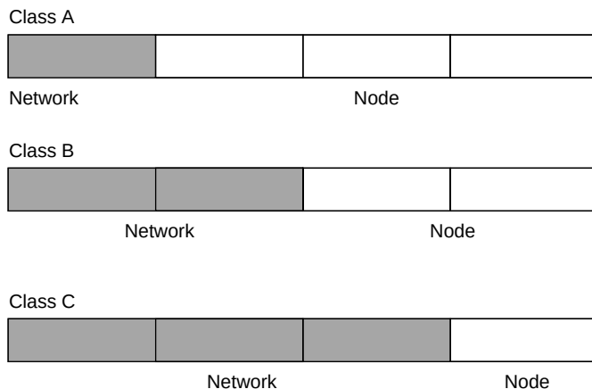
Figure 6-1: Three Main Address Classes
