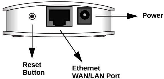
Figure 2-3: WGR101 Rear Panel
