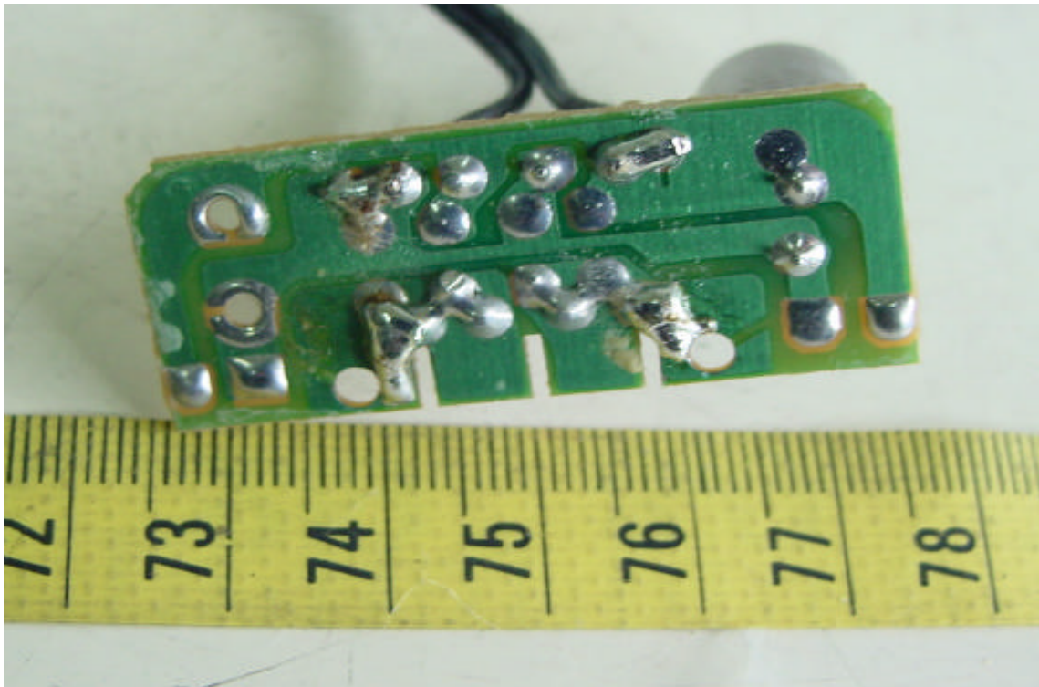
Solder View of Adaptor
