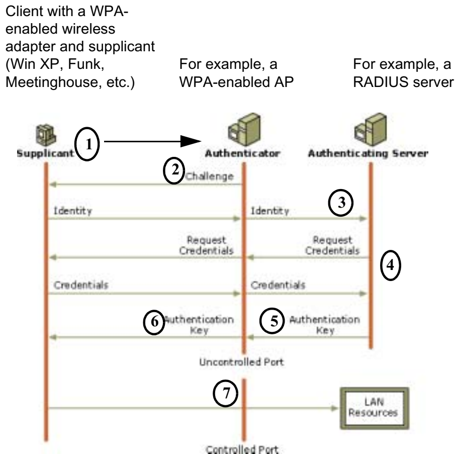
Figure D-4: 802.1x Authentication Sequence
