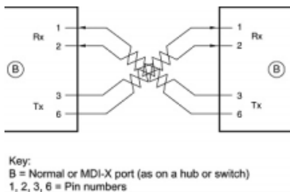
Figure B-5: Crossover Twisted-Pair Cable
