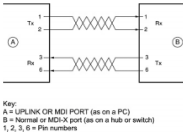
Figure B-4: Straight-Through Twisted-Pair Cable
