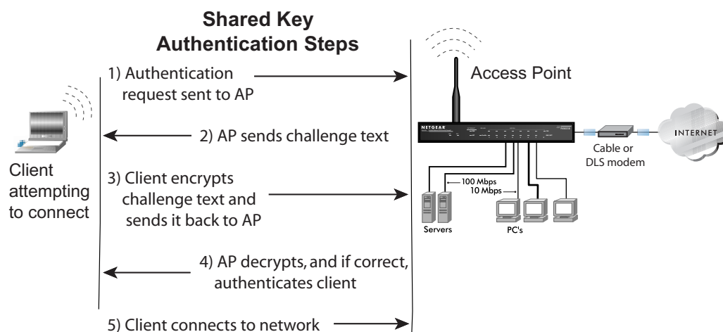
Figure D-2: 802.11 shared key authentication
