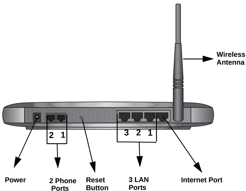
Figure 1-2: wireless router Rear Panel
