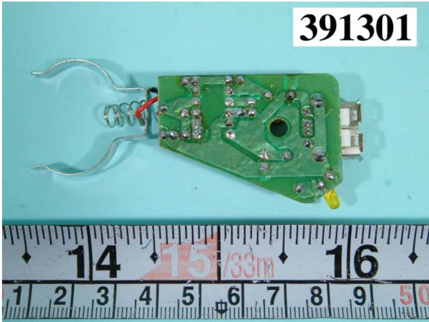
REAR SIDE MAIN BOARD OF DC/DC ADAPTER
