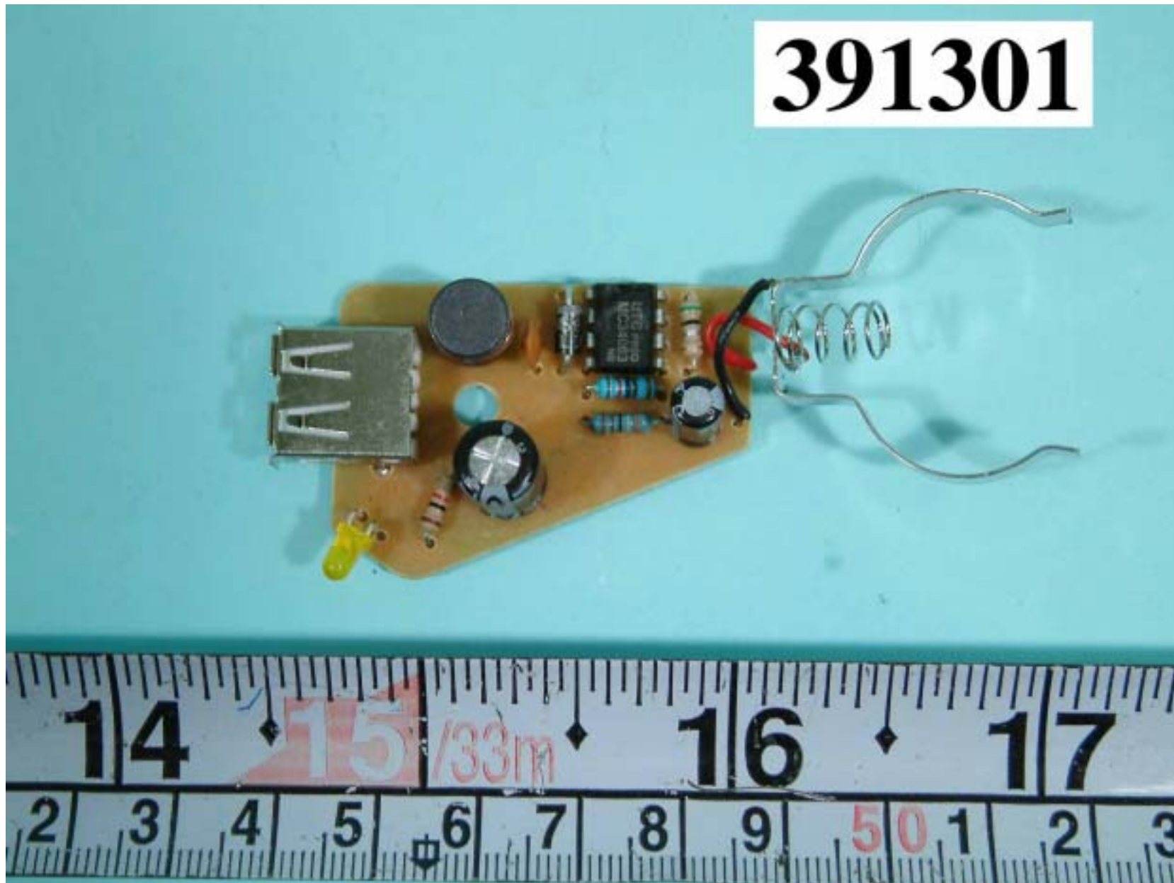
FRONT SIDE MAIN BOARD OF DC/DC ADAPTER
