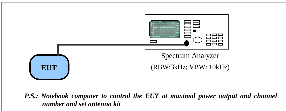
Test Configuration of Power Spectral Density
