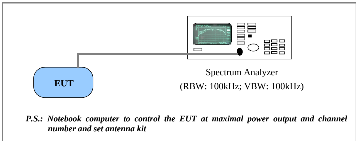
Test Configuration of Bandwidth for Direct Sequence System
