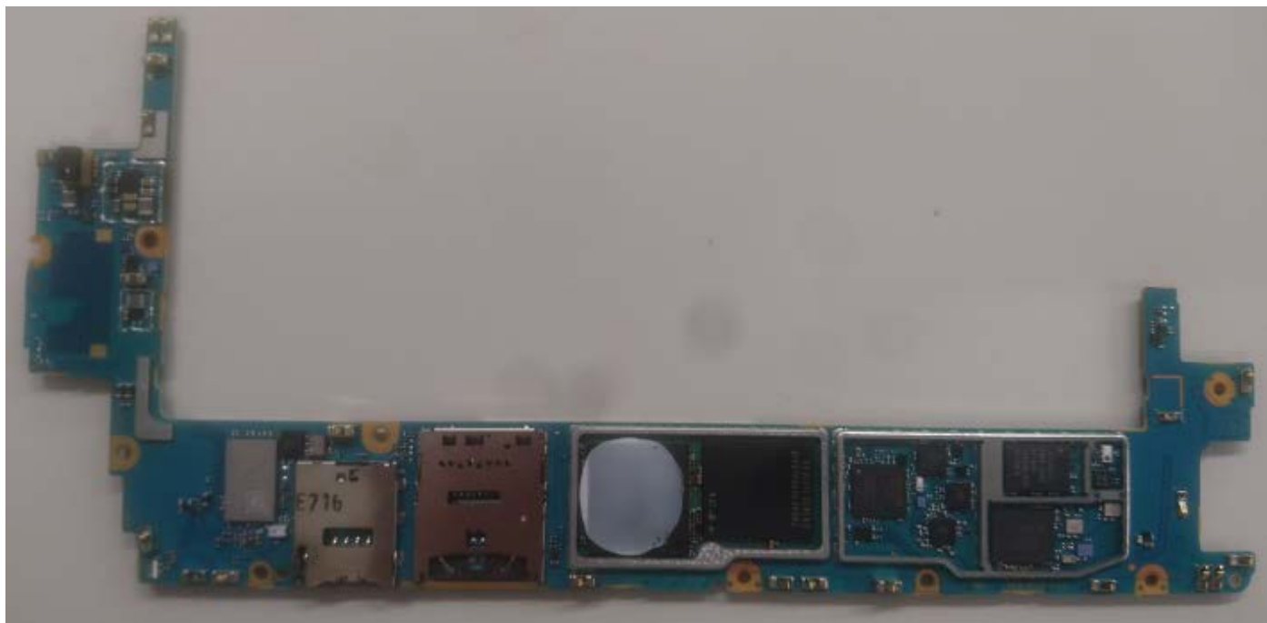
Internal PWB without Shield cases (Front-side)
