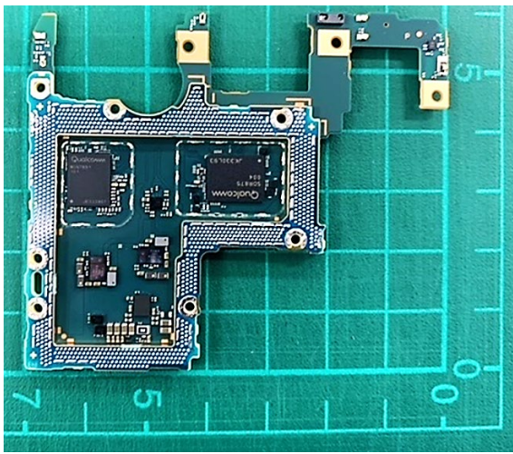
Rear PBA without Shield case (Rear-side)
