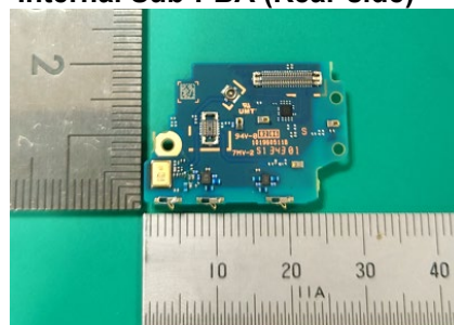
Internal Sub-PBA (Rear-side)
