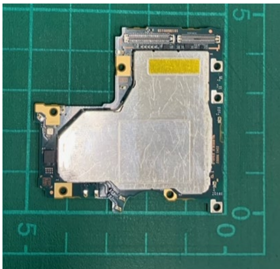
Front PBA with Shield cases (Front-side)
