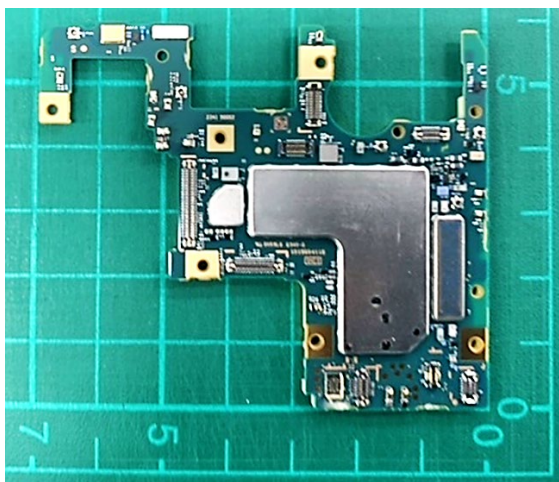
Rear PBA with Shield case (Front-side)
