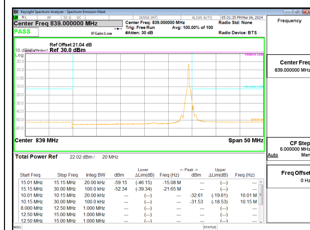
5G NR n5 20MHz BPSK High Channel RB1-104
