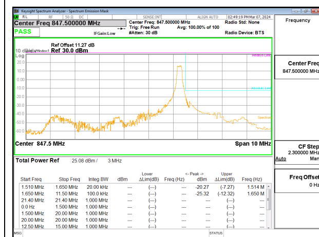
LTE Band 5 3MHz 16QAM High Channel RB1-14
