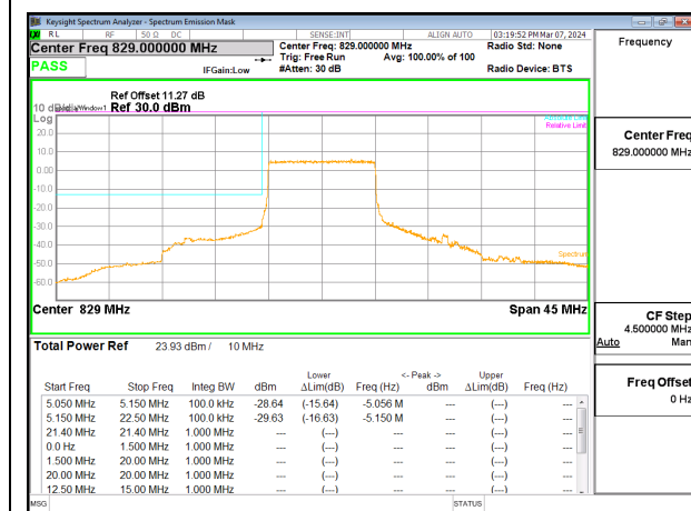
LTE Band 5 10MHz 16QAM Low Channel RB50-0
