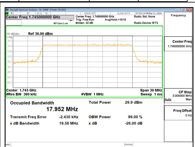
LTE BAND 66 20MHz QPSK MID Ch RB100-0
