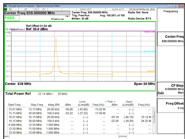
5G NR n5 20MHz BPSK High Channel RB1-0
