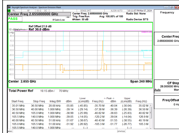
5G NR n41 70MHz QPSK High Channel RB1-70
