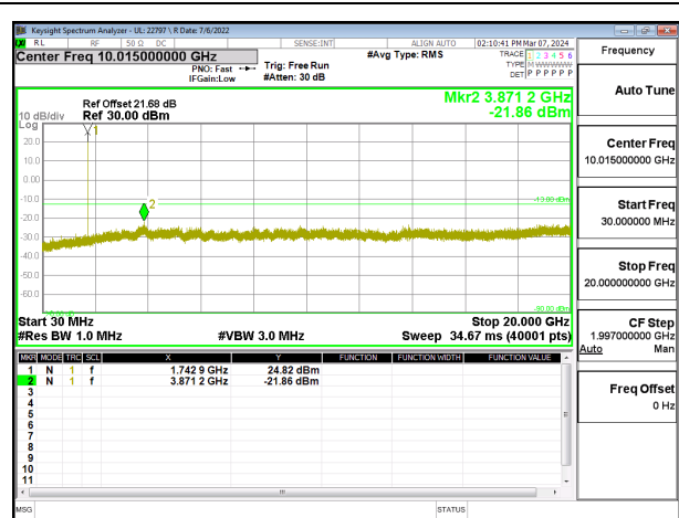
5G NR n66 5MHz BPSK Middle Channel RB1-0
