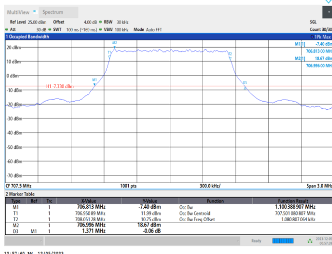
Band12-1.4MHz-16QAM-23095-6RB#0
