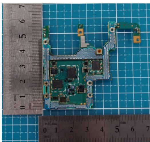
Only ②Rear PBA without Shield case (Front-side)
