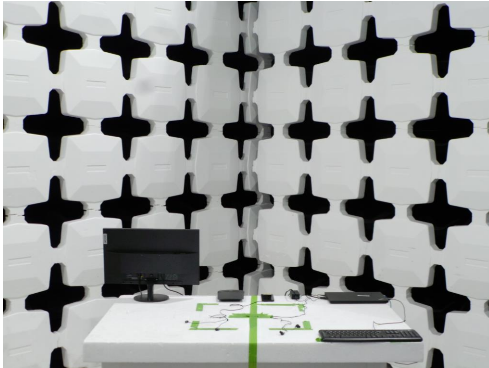
Figure 1. Test setup for Case #1
